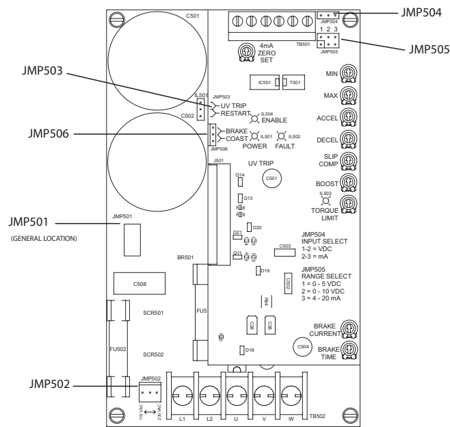
Figure 4. 170-543-0004 Jumper Locations
