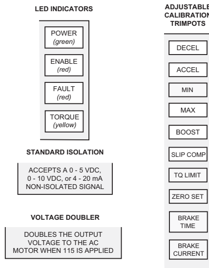
Figure 1. 170-543-0004 Features & Benefits
