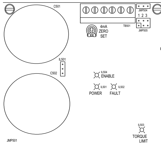
Figure 21. LED locations
