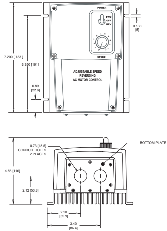
Figure 2. 170-543-0004 Dimensions
