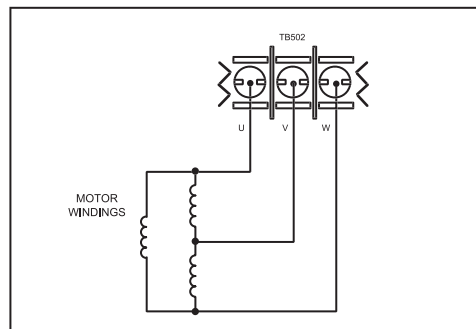
Figure 9. Three-phase Operation
