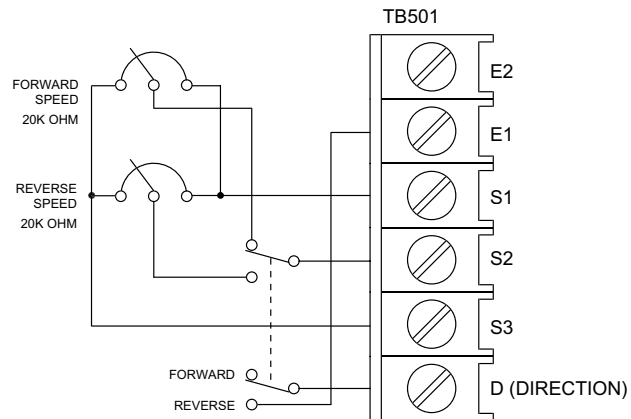
Figure 17. Independent Adjustable Speeds
