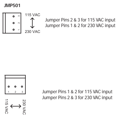
Figure 6. Voltage Doubler Feature for 170-543-0004
