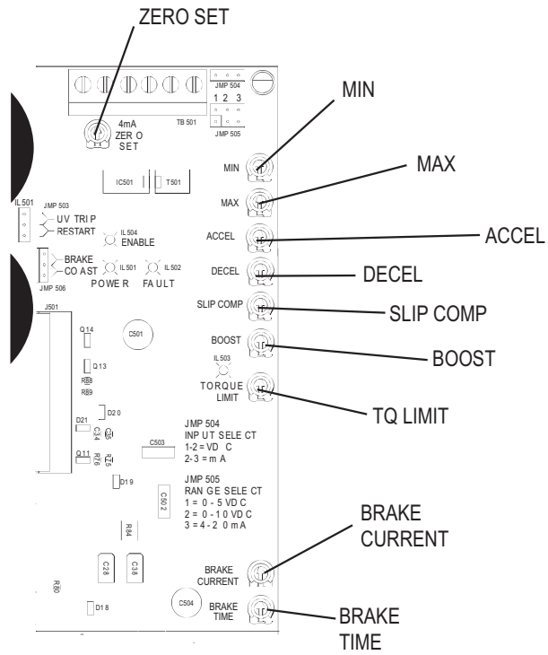
Figure 16. 170-543-0004 Calibration Trimpot Locations
