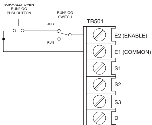
Figure 18. RUN/JOG Switch
