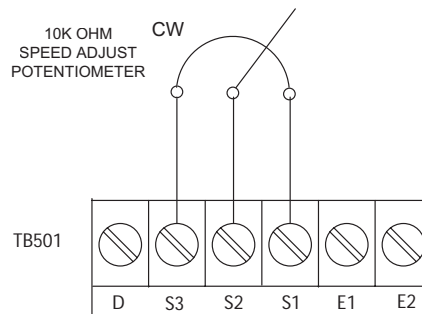
Figure 10. Speed Adjust Potentiometer Connections to TB501
