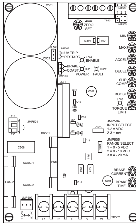
Figure 3. 170-543-0004 Circuit Board Layout
