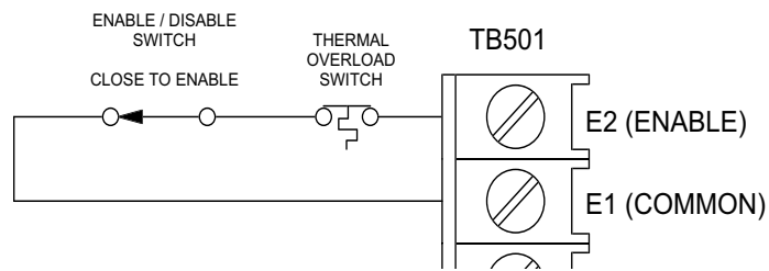
Figure 14. Thermal Overload Switch with Optional Enable / Disable Switch
